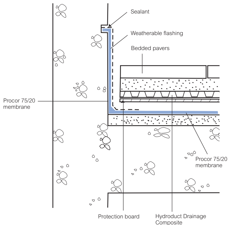
Typical Deck Upstand Detail
