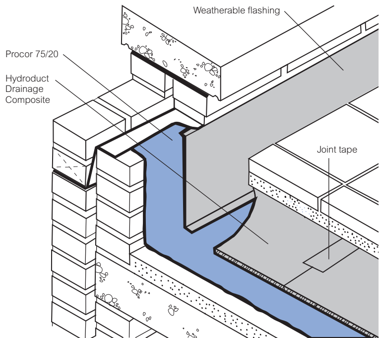
Typical Elevated Deck Waterproofing
